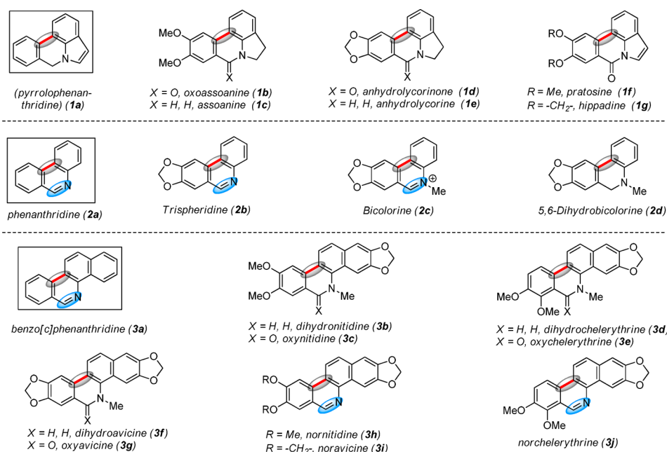
Figure 1. Alkaloids sharing pyrrolophenanthridine, phenanthridine, and benzo[ c ]phenanthridine structures.
