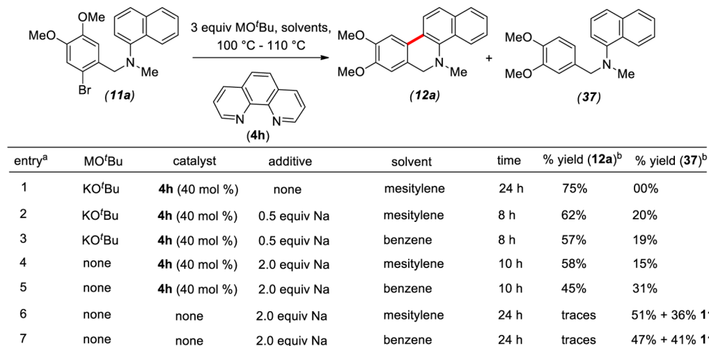
Scheme 10. Biaryl-Coupling in the Presence of Na-Metal as a Reducing Agent a
