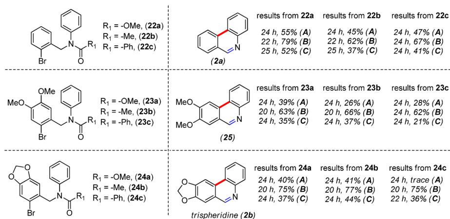
Figure 7. One-pot deprotection, biaryl-coupling followed by oxidation.
