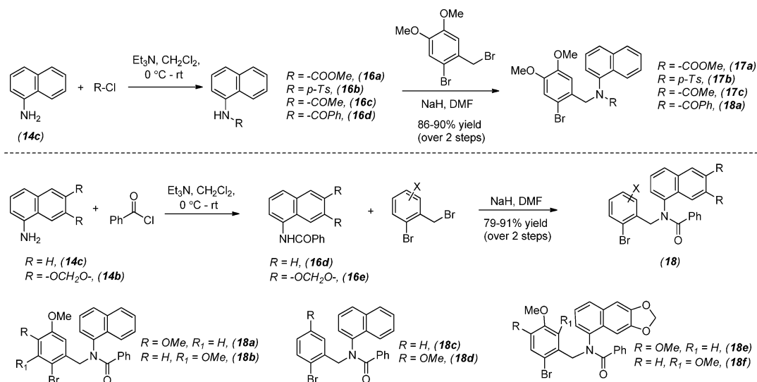
Figure 5. Synthesis of dihydronitidine, avicine, and chelerythrine.
