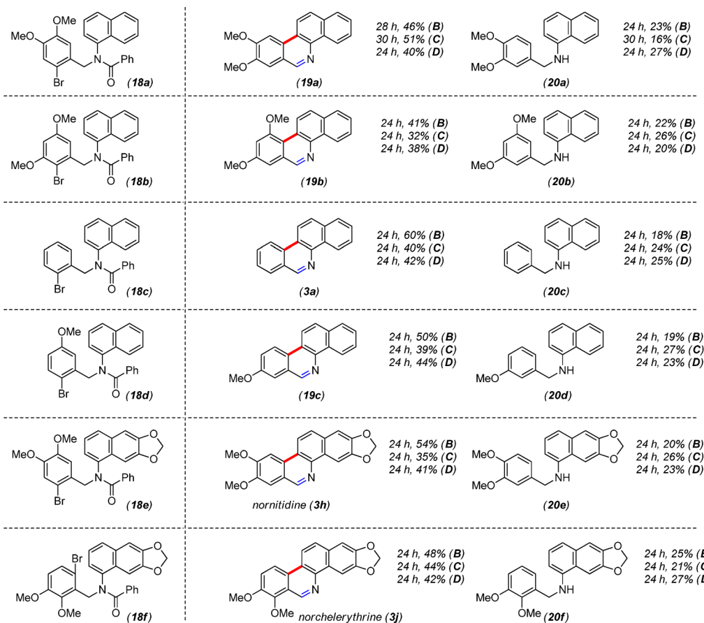
Figure 6. One-pot debenzoylation, biaryl-coupling followed by oxidation sequence.
