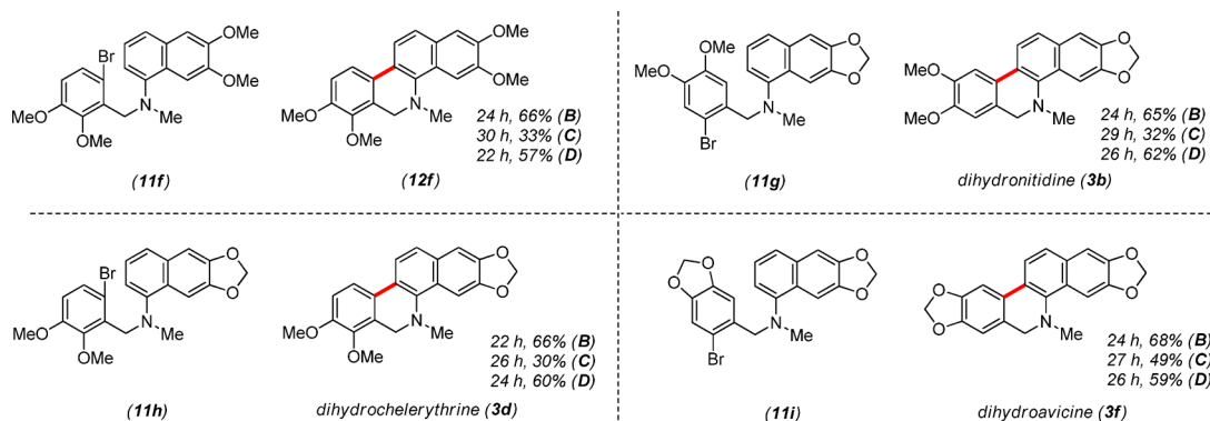
Figure 5. Synthesis of dihydronitidine, avicine, and chelerythrine.
