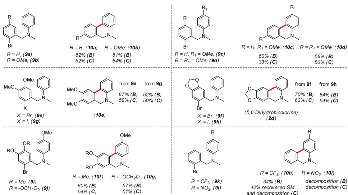
Figure 3. Substrate scope of dihydrophenanthridine synthesis. a Reactions were carried out on a 1.0 mmol of 9a–l in presence of 0.50 mmol of 4h (condition B) and 3.0 mmol of KO t Bu in 6 mL of solvent in a sealed tube at 100 °C for 24 h. Condition C = 3.0 mmol of KO t Bu only.
